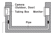
Stop up P.V.C pipe using adiabatic substances, to prevent air circulation
